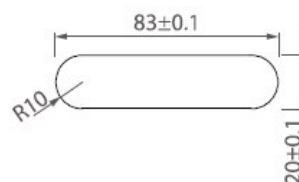
drilling template
